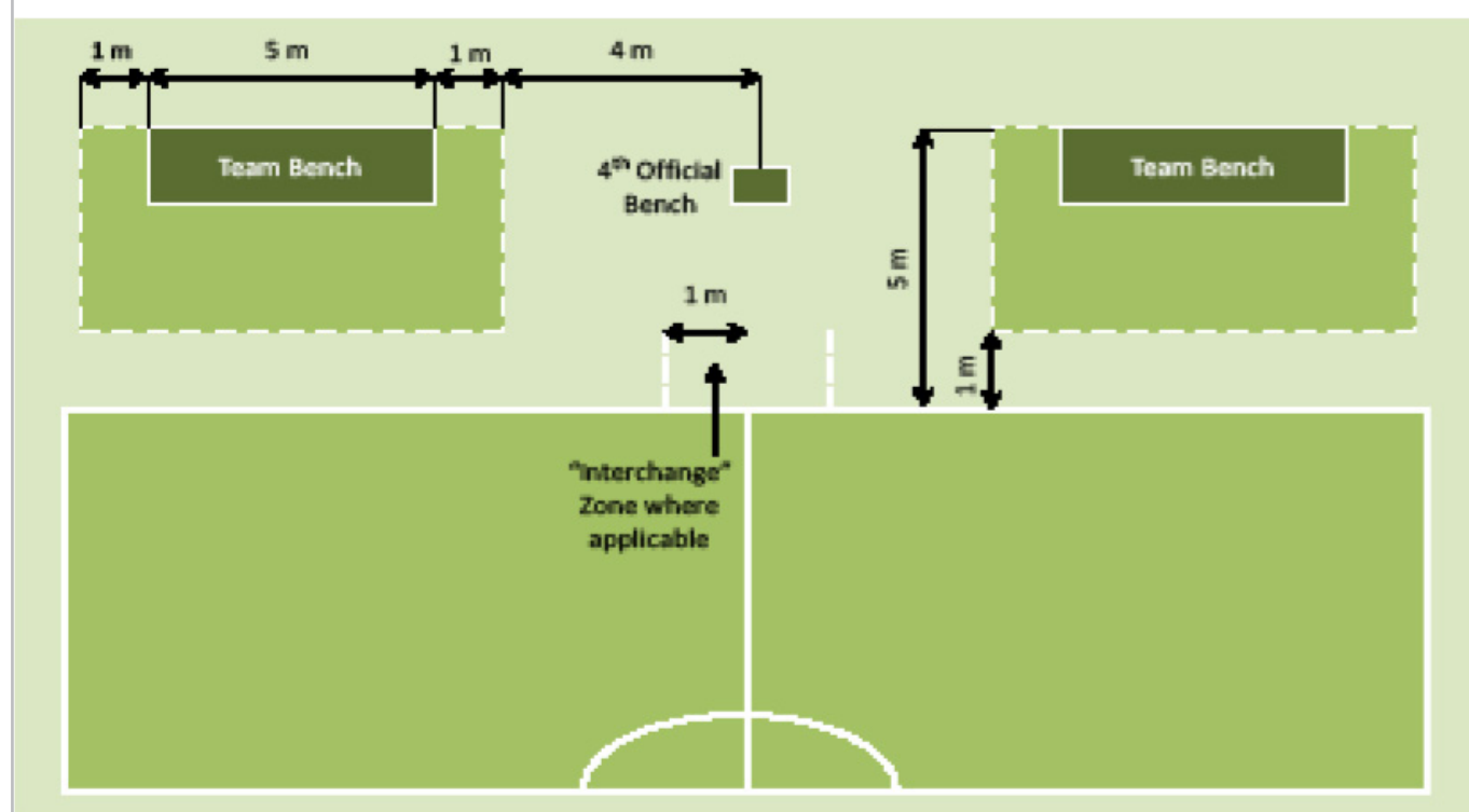
Diagram 6 - Technical Area line marking and dimensions
