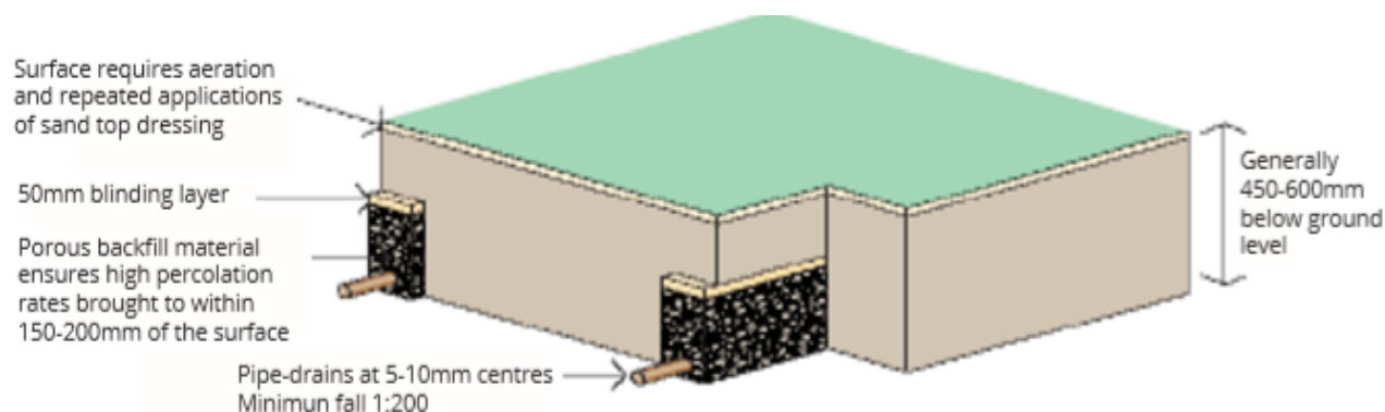
Diagram 2 - Pipe drainage construction
